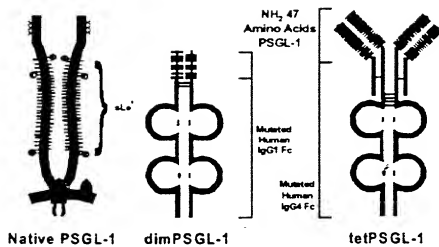
Structure of PSGL-1 Molecules
